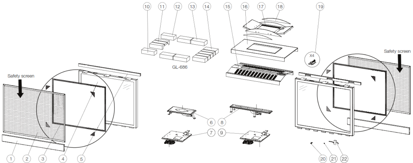
GLASS BURNER ASSEMBLY
